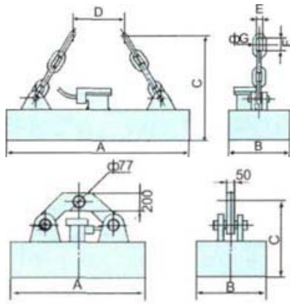
overall dimension sketch
