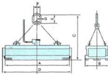
overall dimension sketch
