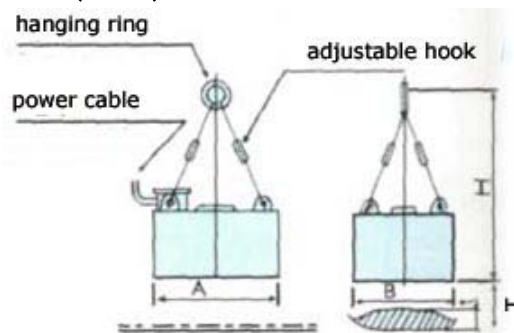
overall dimension sketch
