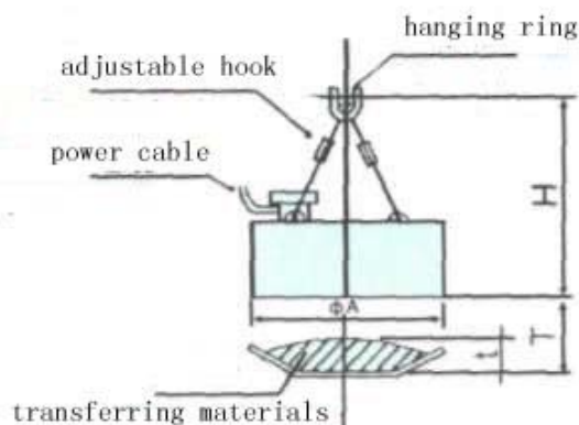
overall dimension sketch
