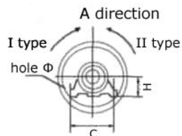
RCTG series permanent magnetic pulleys appearance size and installation size sketch map
