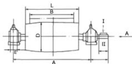
RCTG series permanent magnetic pulleys appearance size and installation size sketch map
